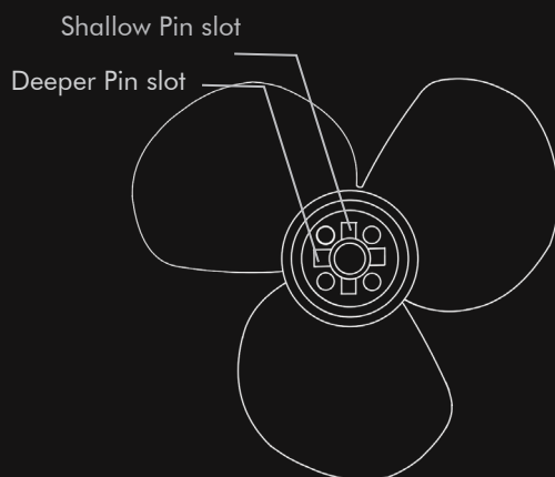
3 blades propeller
